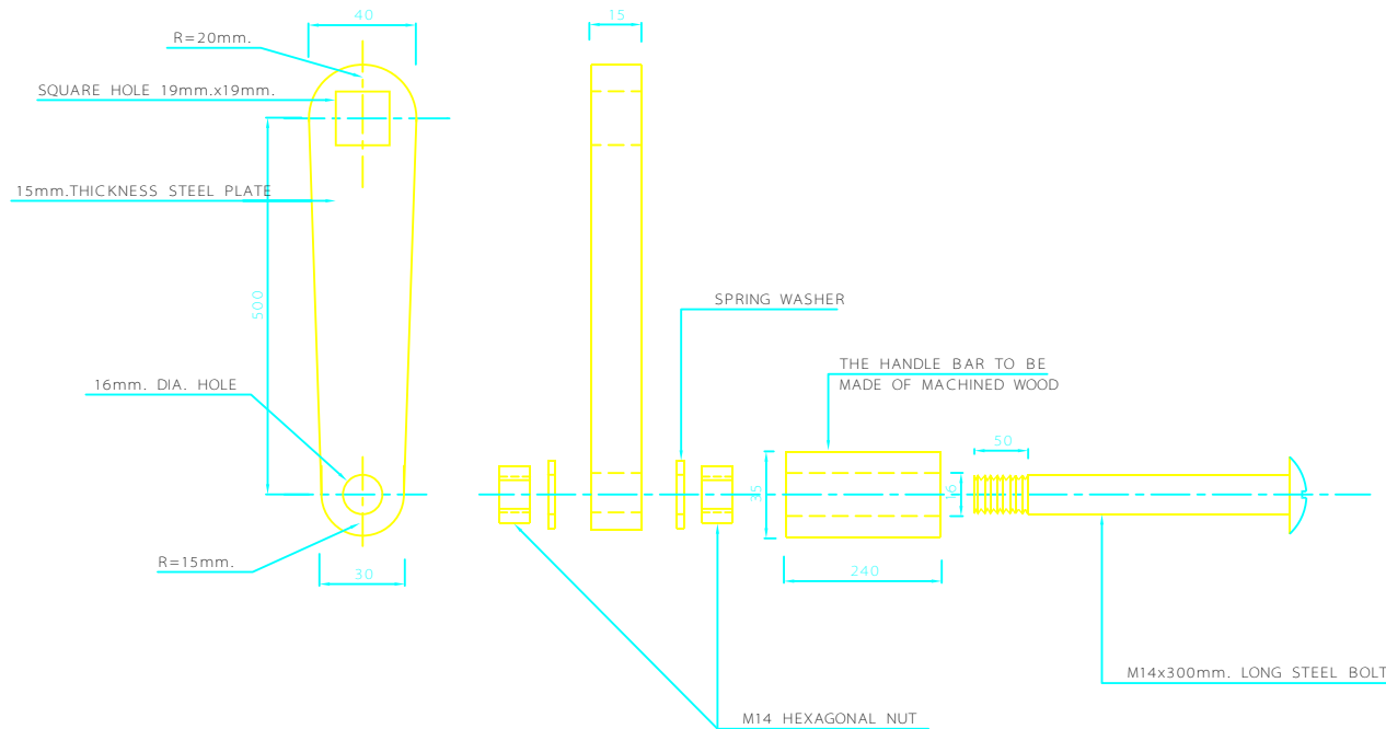
3 - WINDING HANDLE
