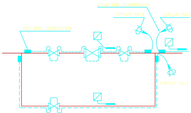
ELECTRIC HEAT TRACING FOR TANK
