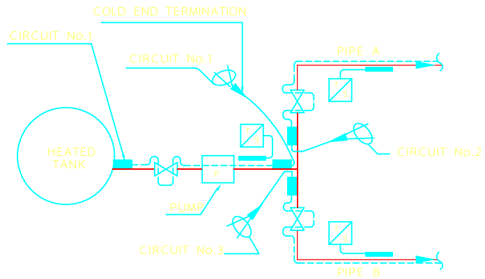
ELECTRIC HEAT TRACING FOR TANK
