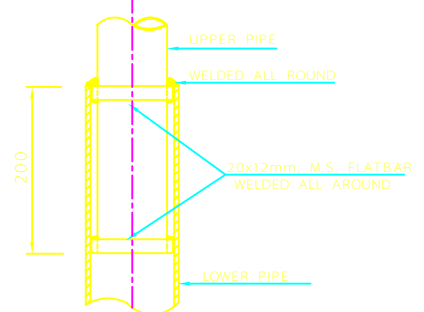
DETAIL "A" PIPE CONNECTION
