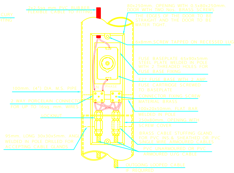
DETAIL "B" CABLE CONNECTION INSIDE THE POLE
