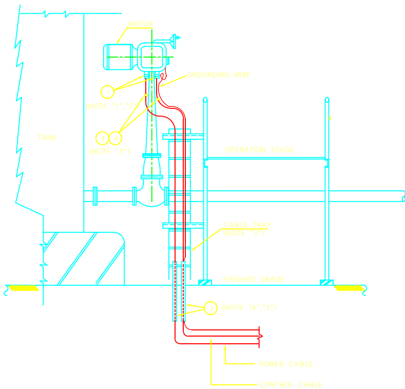
MOTOR OPERATED VALVE FEEDER & CONTROL
