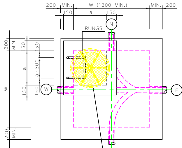
GREY CAST IRON AIRTIGHT PEDESTRIAN COVER FOR 600 DIA. M.H. ENTRANCE
