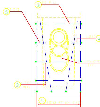
END ELEVATION (AT OUTLET PIPE SIDE)
