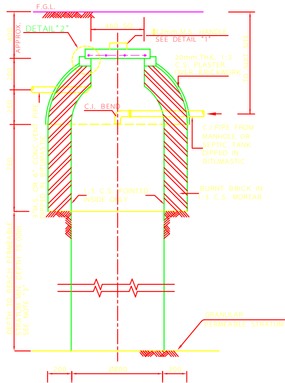
SOAKAWAY PIT (SECTIONAL ELEVATION)
