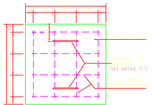
DETAIL OF PRECAST CONC. COVER SLAB (FOR SOAKAWAY PIT)
