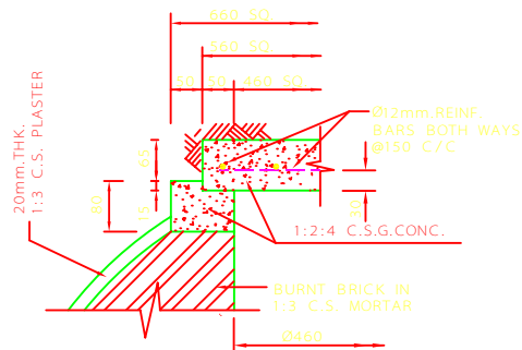
DETAIL "2"
