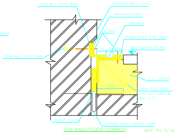
FOR WALL/FLOOR CORNERS NOT TO SCALE
