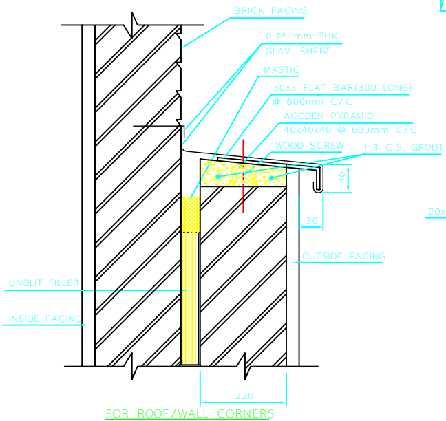
FOR ROOF/WALL CORNERS
