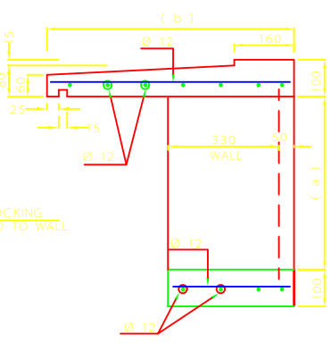
LONG SECTION
