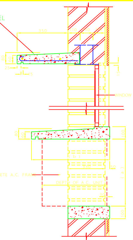
UNDER WINDOW SILL (WITH CONCRETE FRAME)
