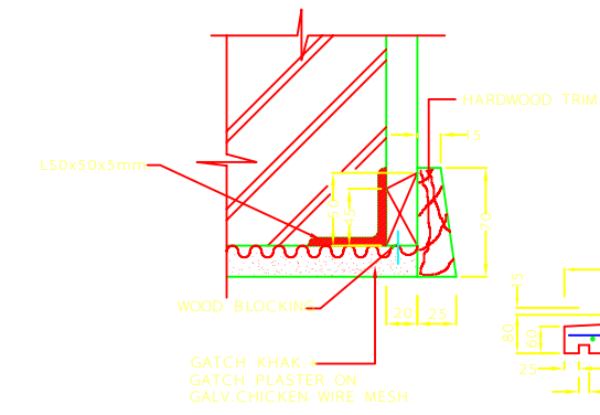
DETAIL " A "
