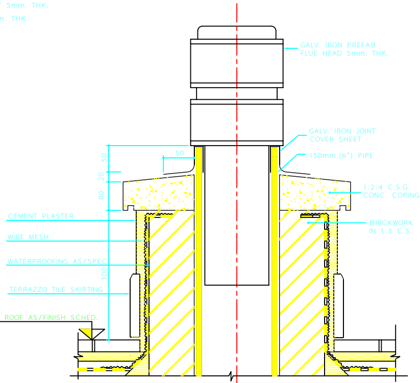
SECTIONAL VIEW (CHIMNEY WITH CONCRETE COPING)
