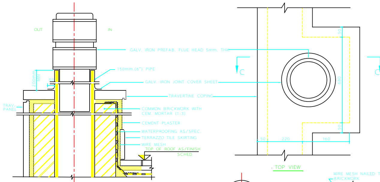
SECTION C-C CHIMNEY WITH TRAVERTINE COPING (ADJACENT TO PARAPET WALL)
