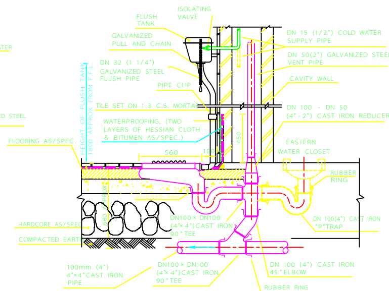
EASTERN WATER CLOST (GRADE LEVEL)
