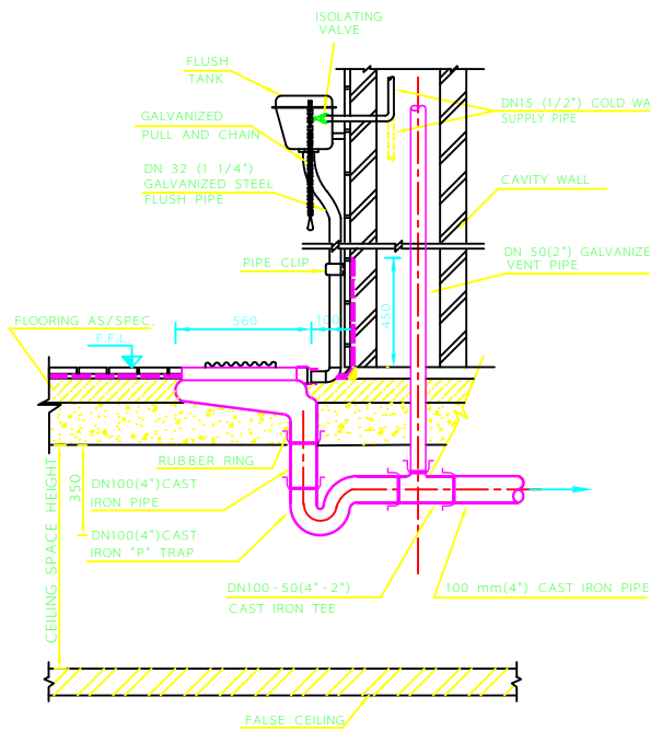
EASTERN WATER CLOSE (ABOVE GRADE)
