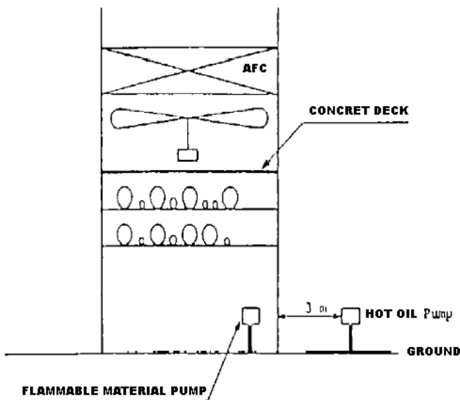
LAYOUT OF FLAMMABLE MATERIAL PUMPS
