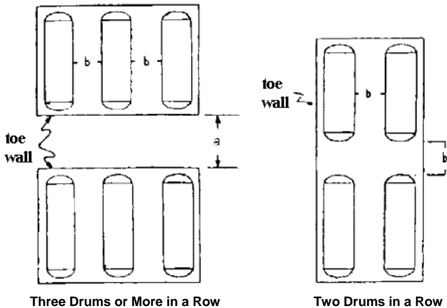
SPACING BETWEEN HORIZONTAL VESSELS/DRUMS Fig. 6
