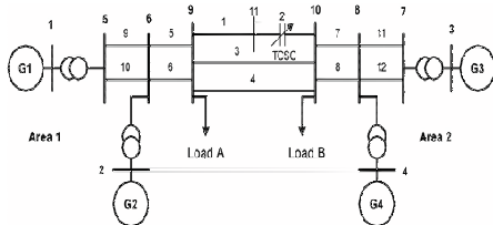
Fig. 3. Two area four machines power system with TCSC
